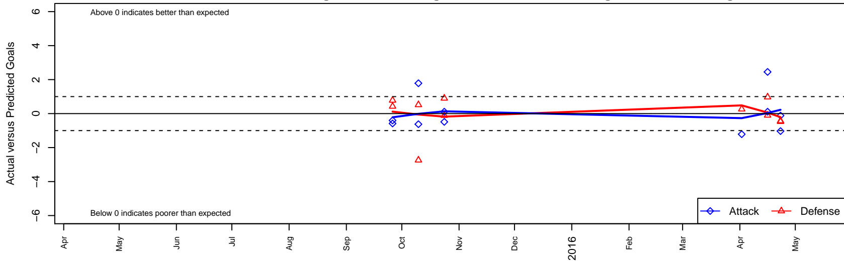
UC United G01 Dots are actual minus expected GF (blue circles) and GA (red triangles). Blue line is smoothed change in attack strength. Red is smoothed change in defense strength.
